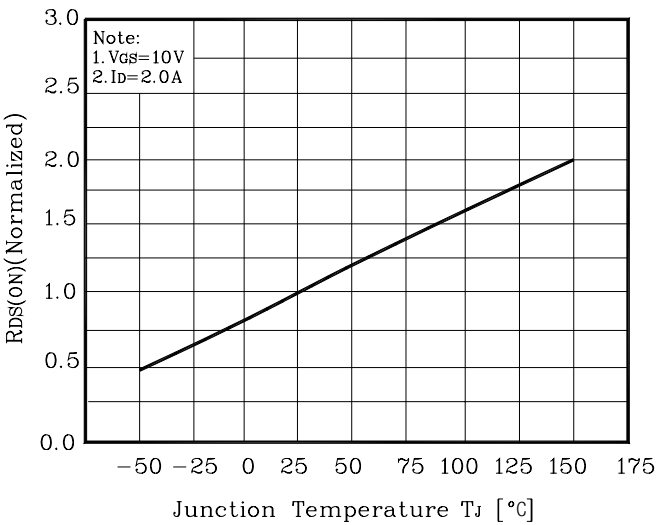
Fig. 8 R_{DS(on)} - T_J
