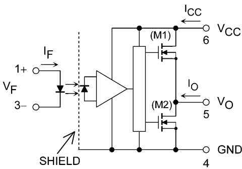
Fig. 5.1 Internal Circuit
